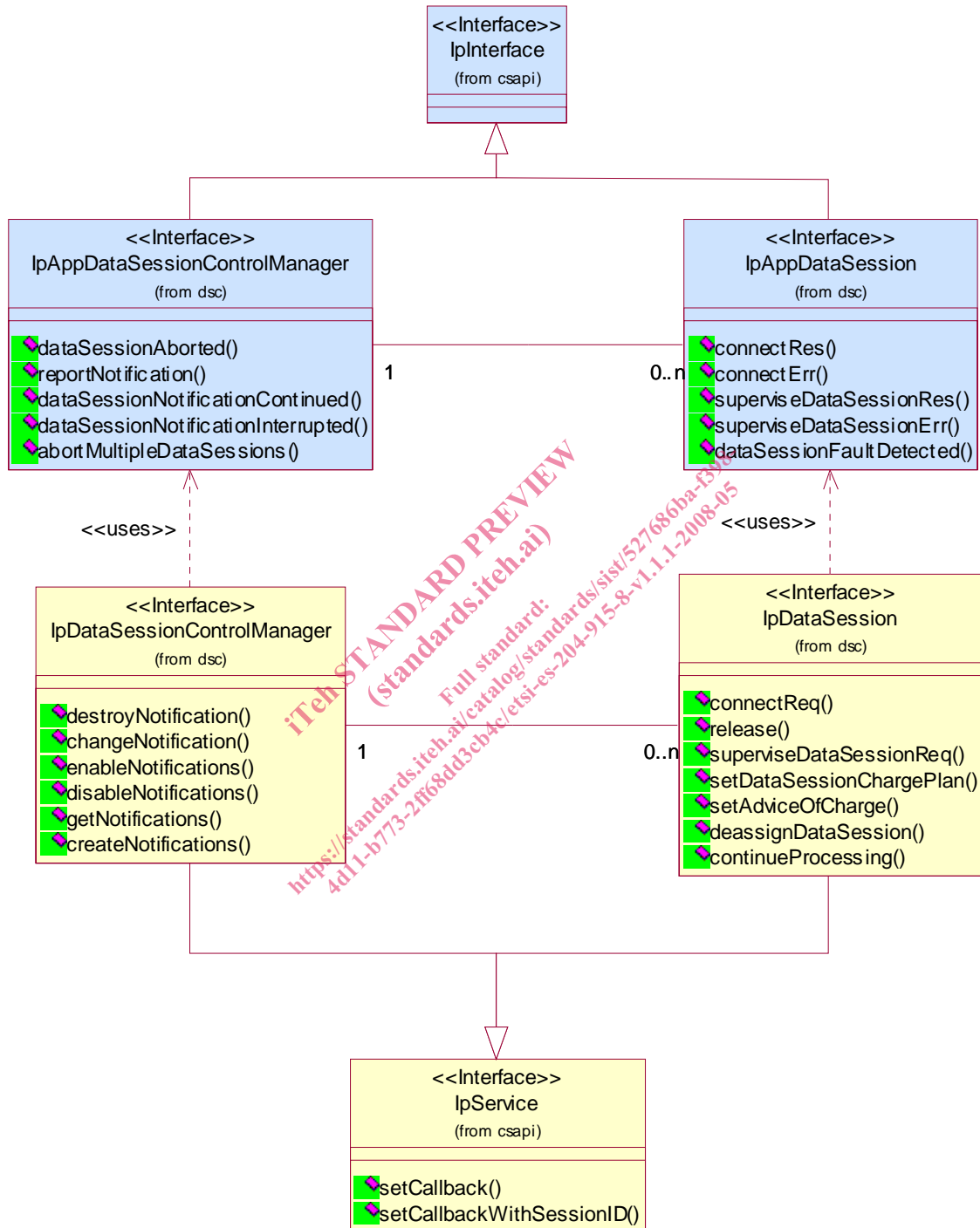
Figure 2: Package Overview
