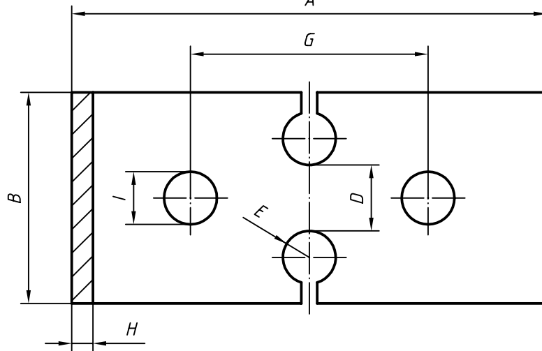
Figure 1 — Machined type A tensile test piece (for e < 25 mm)
