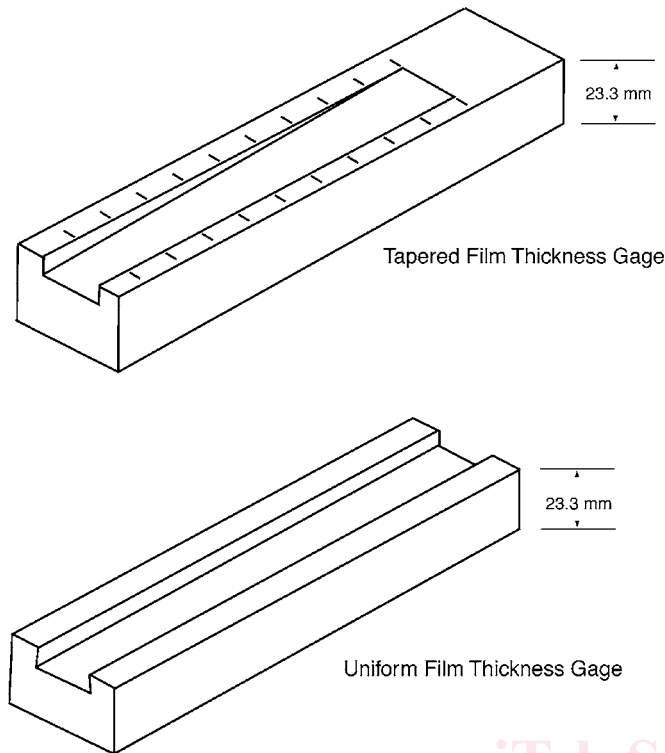
FIG. 1 Schematic Diagram of Printing Gages (not drawn to scale)
