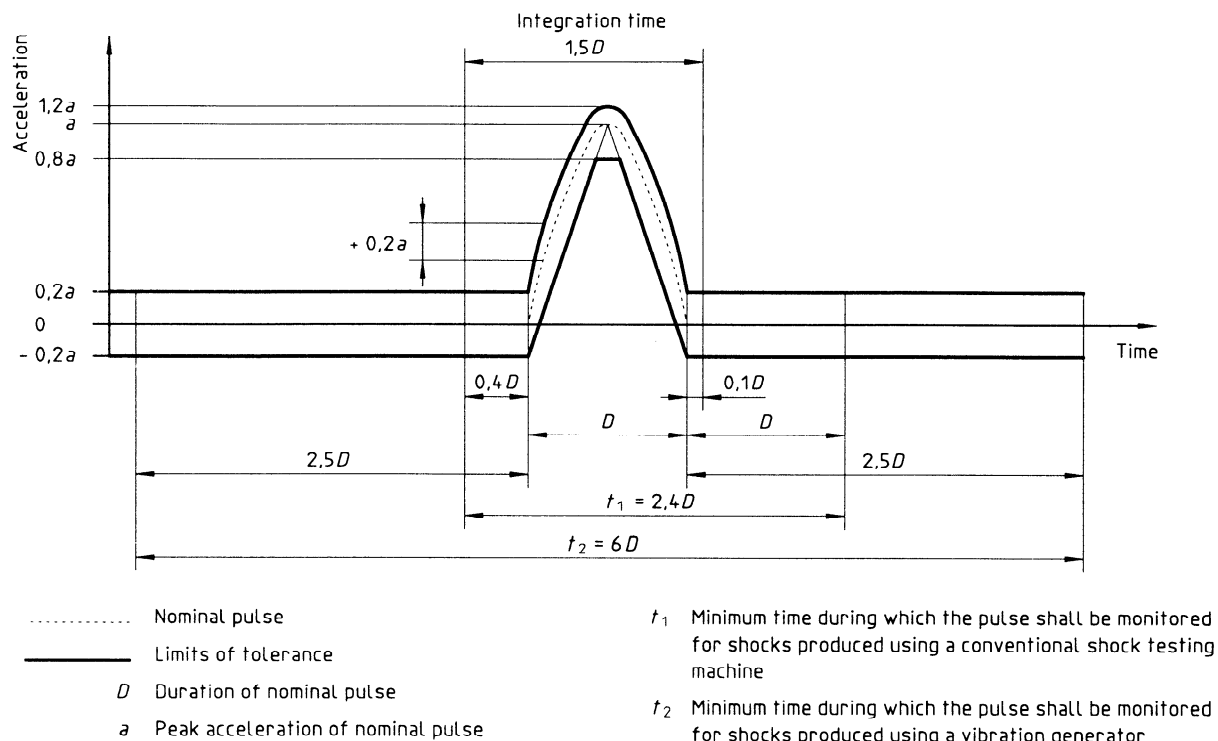
Figure 3 — Half-sine pulse
