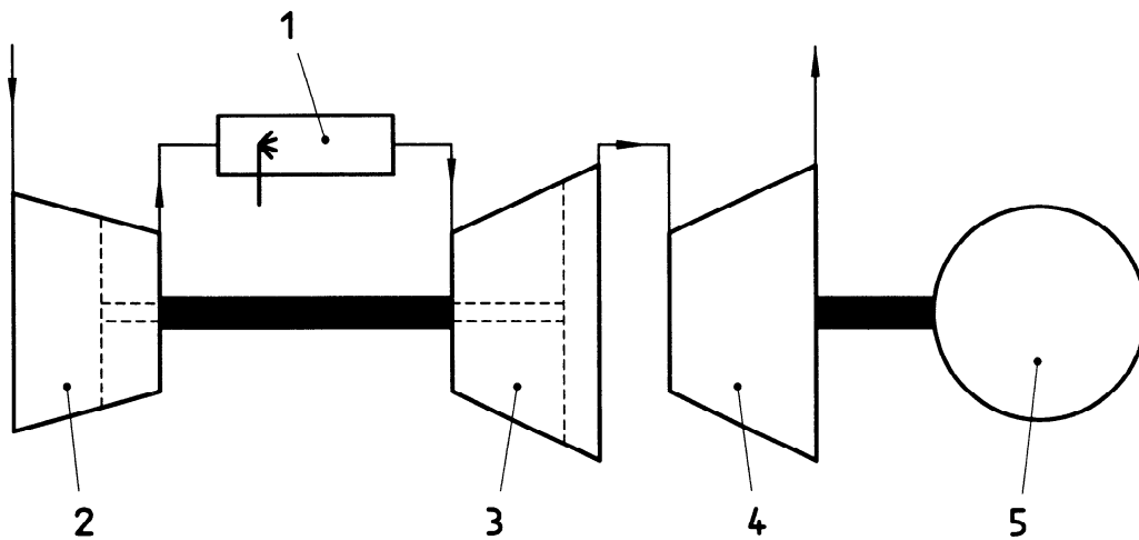
Figure 2 — Regenerative cycle, single-shaft gas turbine https://standards.iteh.ai/catalog/standards/sist/10531260-c11c-4ac1-b298-a24327fc1482/iso-3977-1-1997
