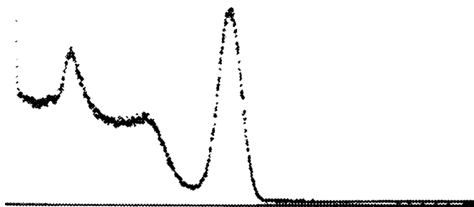
FIG. 4 The Gamma-Ray Spectrum of ^{137}\text{Cs} Detected by a NaI(Tl) Scintillator and Viewed with a Multi-Channel Analyzer
