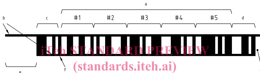
Figure 1 – "Code 16K" row structure https://standards.iteh.ai/catalog/standards/sist/09eecd8c-2c63-4ec0-91b1-c6fb02b4378e/sist-en-12323-2005
