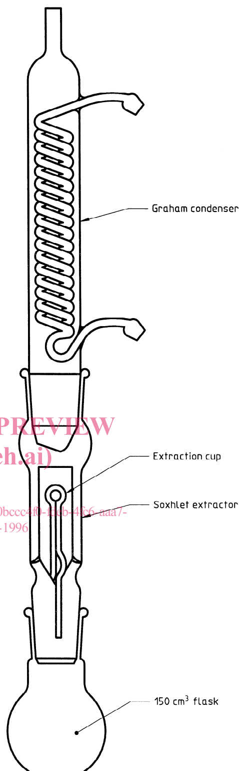
Figure 1 — Extraction apparatus
