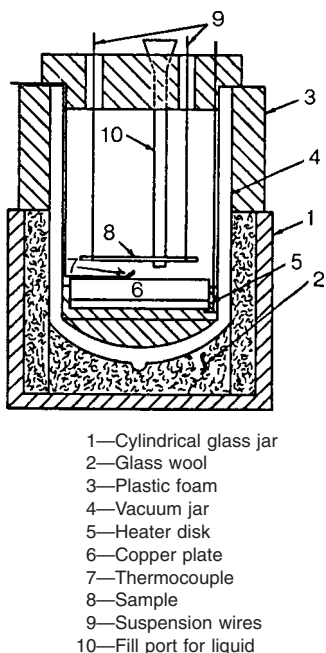
FIG. 2 Detail Drawing of a Typical Cryogenic Chamber
