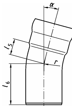
Figure 4 — Shape C 1
