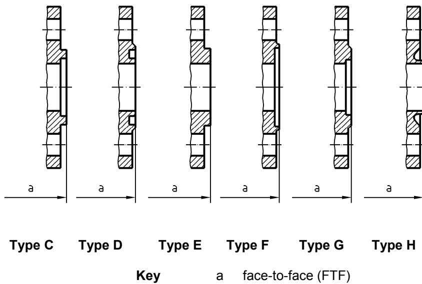
Figure 3 - Flanged valves PN designated (spigot and recess)
