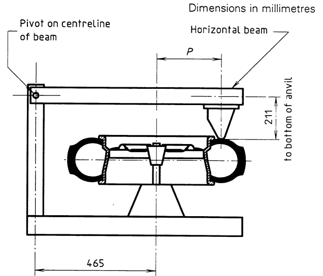
Figure 2 — Bead unseating fixture
