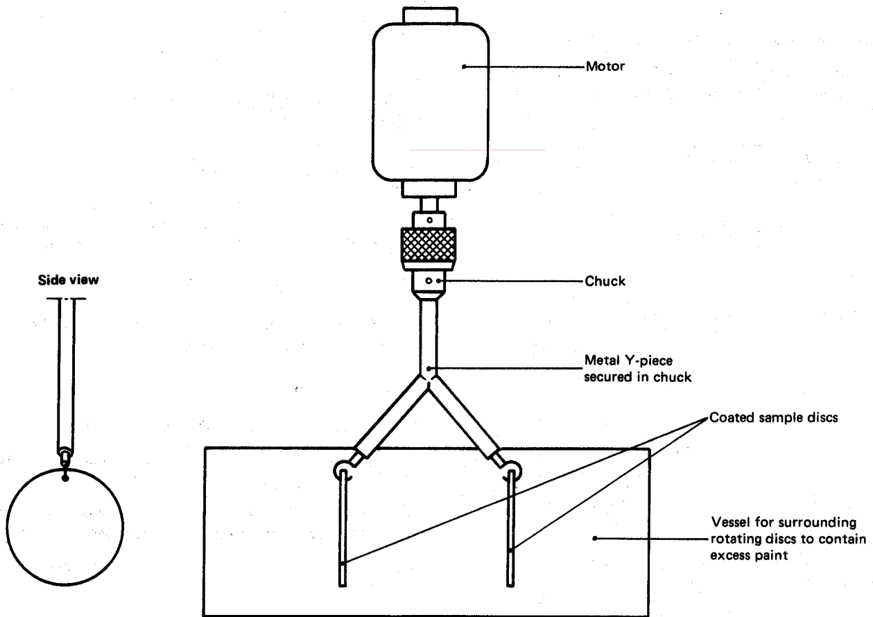
FIGURE 2 — Device for centrifuging discs to ensure a uniform coating of paint
