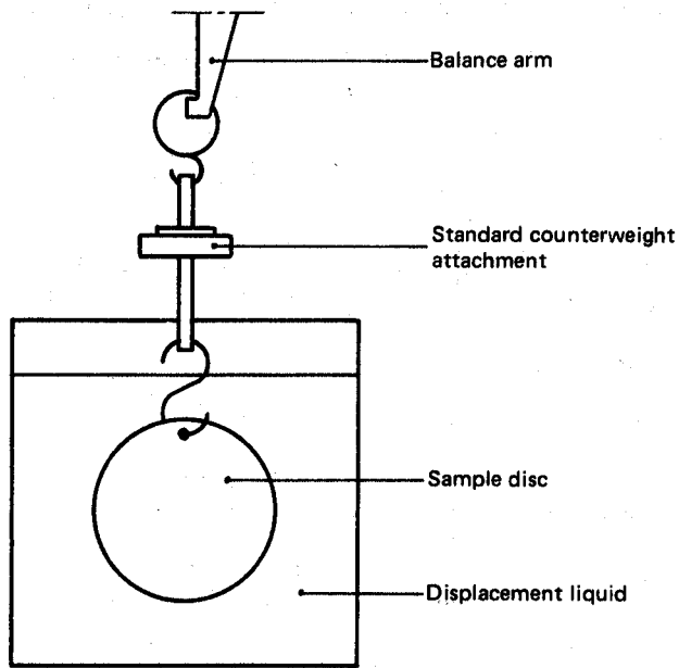
FIGURE 1 — Special balance support
