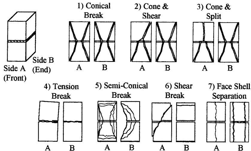
FIG. 4 Sketches of Types of Fracture
