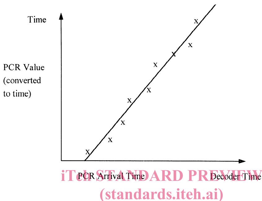
Figure 2 - Plot of PCR values versus Arrival Time
