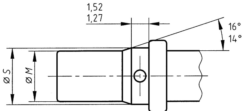
Figure 2 – Barrel, contact sizes 16-18
