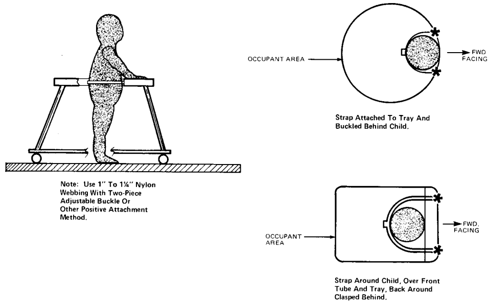
FIG. 4 Placement of CAMI Infant Dummy
