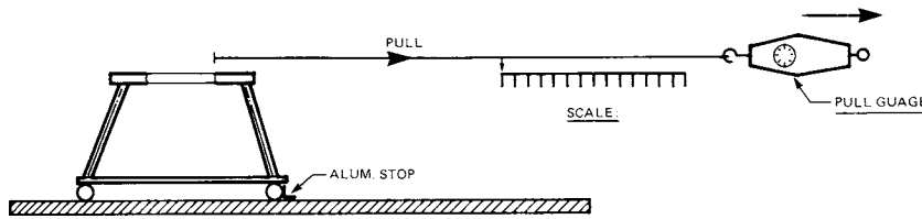
FIG. 5 Tip Resistance Setup
