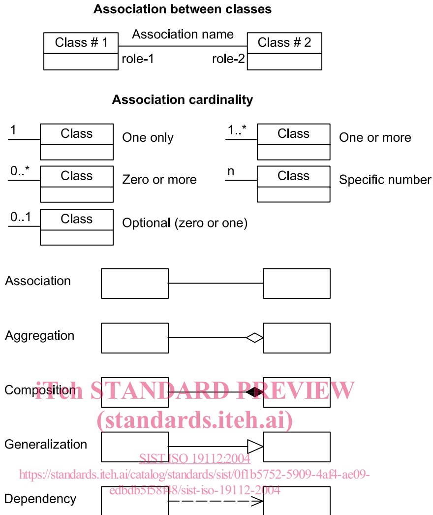
Figure 1 — UML notation
