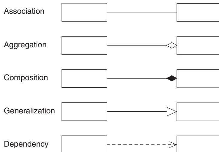
Figure 1 — UML notation
