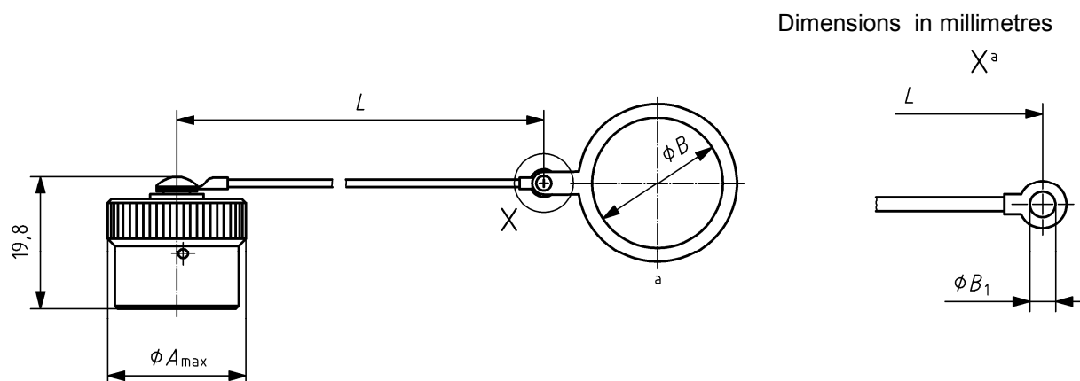
Figure 1 — Protective cover Table 1 — Dimensions and mass
