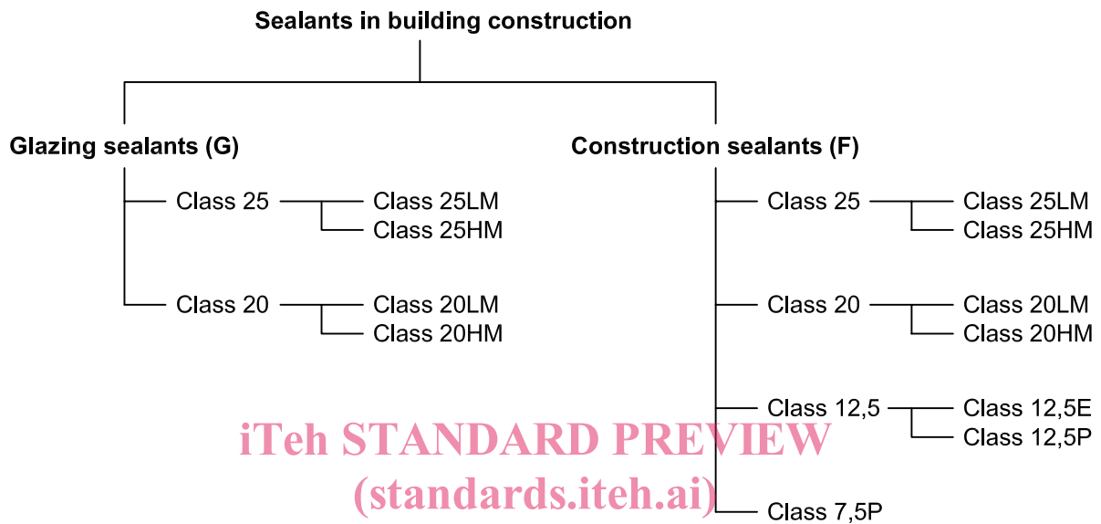
ISO 11600:2002 Figure 1 — Diagram of classification of sealants in building construction https://standards.iteh.ai/catalog/standards/sist/61a862a1-a45e-4a55-96cd-afe0b60d57a2/iso-11600-2002
