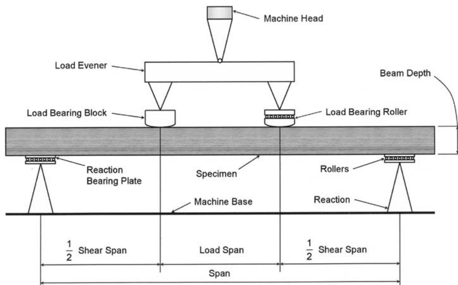
FIG. 1 Flexure Method
