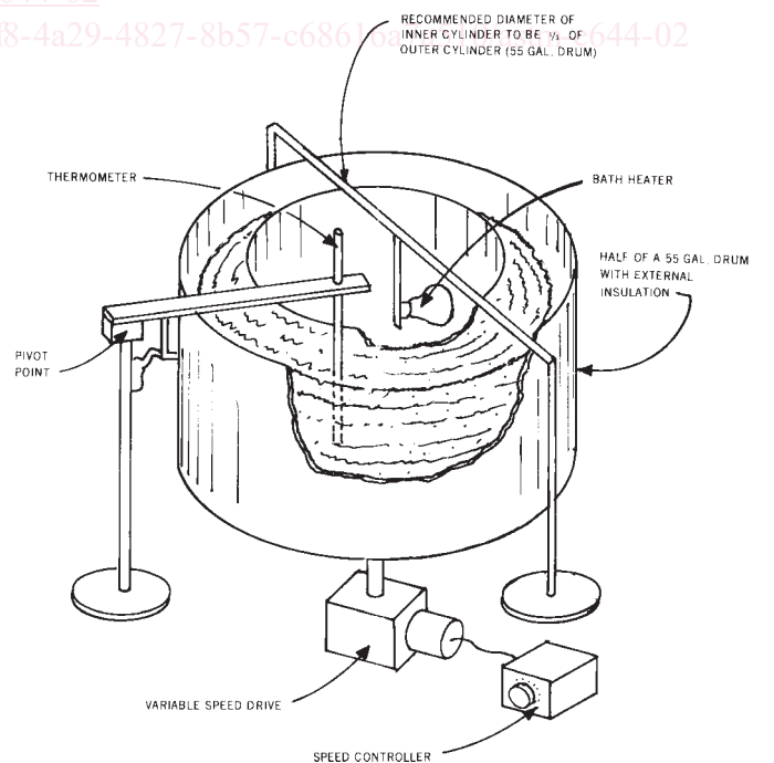
FIG. 3 Typical Bath Arrangement
