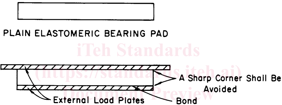
PLAIN ELASTOMERIC SANDWICH BEARING
