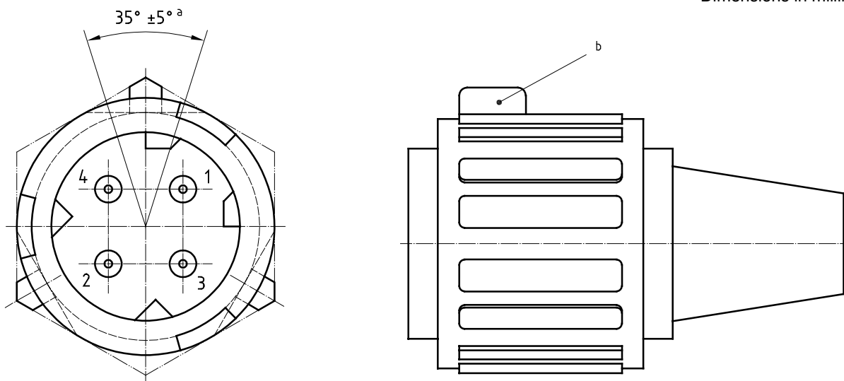
a) Marking zone at fixed or free connector
