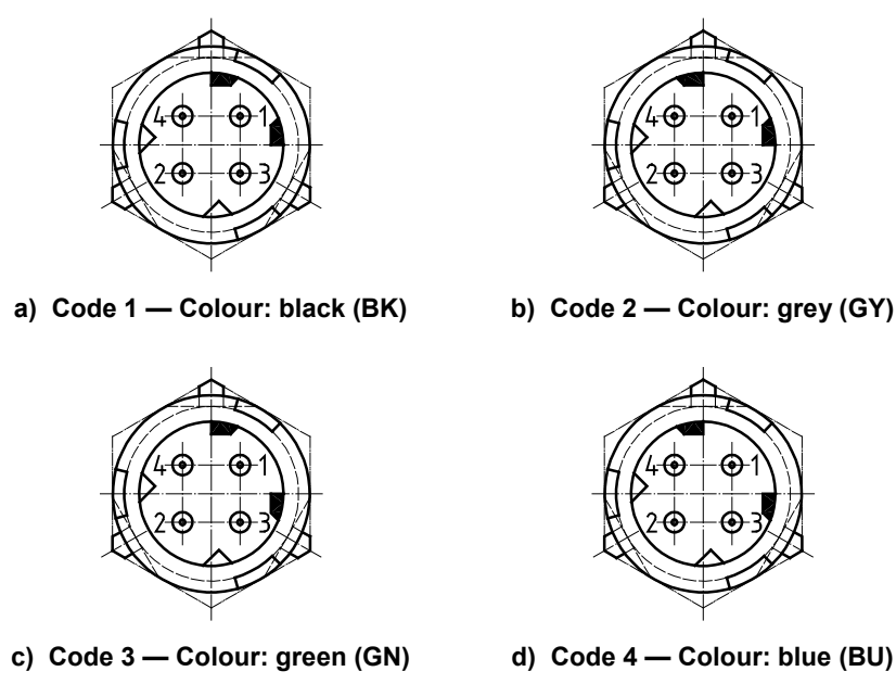
Figure 4 — Mechanical and colour coding
