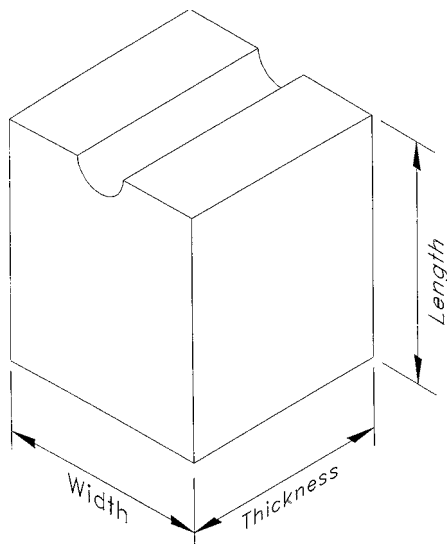
FIG. 1 Specimen Configuration
