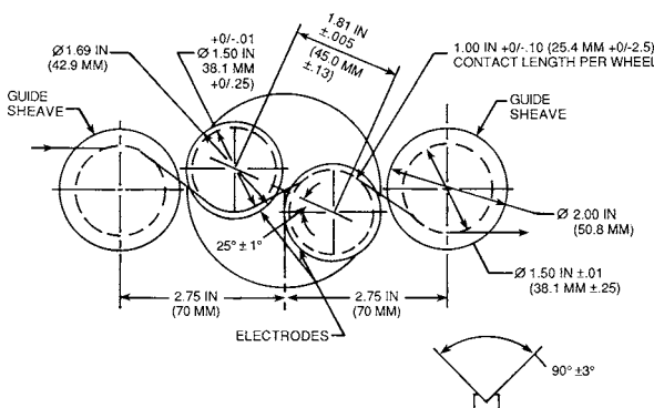
FIG. 7 Direct-Current High Voltage Continuity Electrodes for Wire Sizes 14 to 30 AWG 0.0641 to 0.010 in. (1.628 to 0.254 mm)
