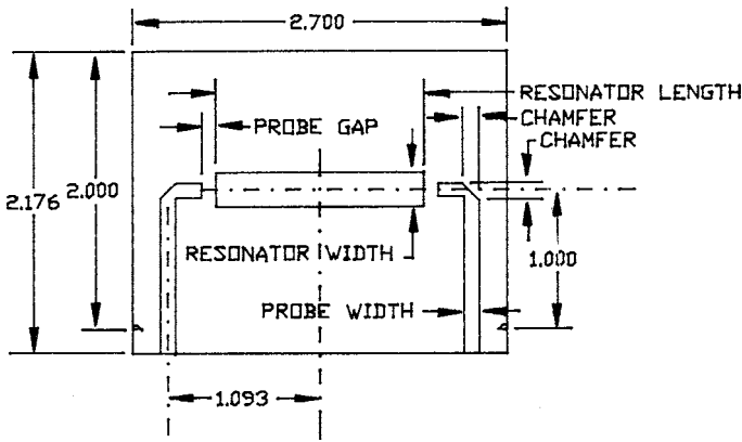
FIG. 8 Generalized Resonator Pattern Card for Fixture A Showing Dimensions of and Made of Laminate Matching the Nominal Permittivity of Materials to be Tested
