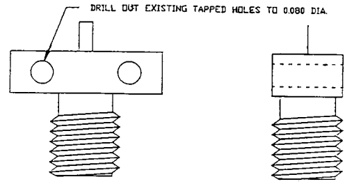
FIG. 11 Detail of the Supplied End Launcher Body Adapted by Boring Out the Tapped Holes
