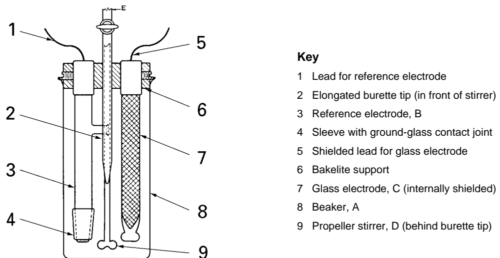
Figure 1 — Typical titration cell assembly
