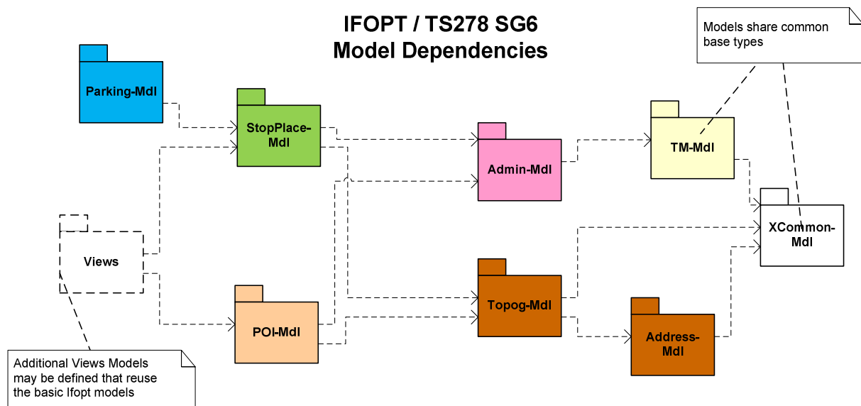
Figure 2 — Dependencies of Fixed Object Models
