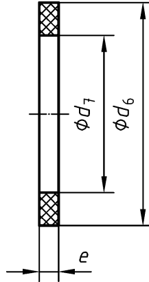
Figure 8 – Gasket
