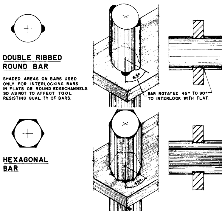
FIG. 1 Shaped Bars
