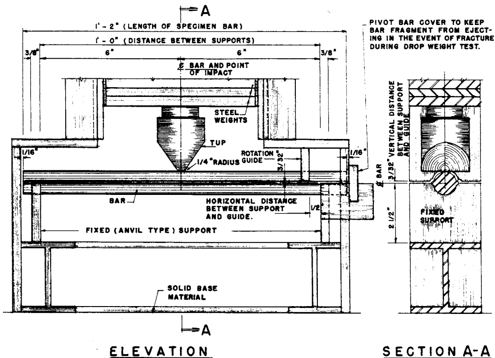
FIG. 2 Typical Example of Drop-Weight Test Apparatus
