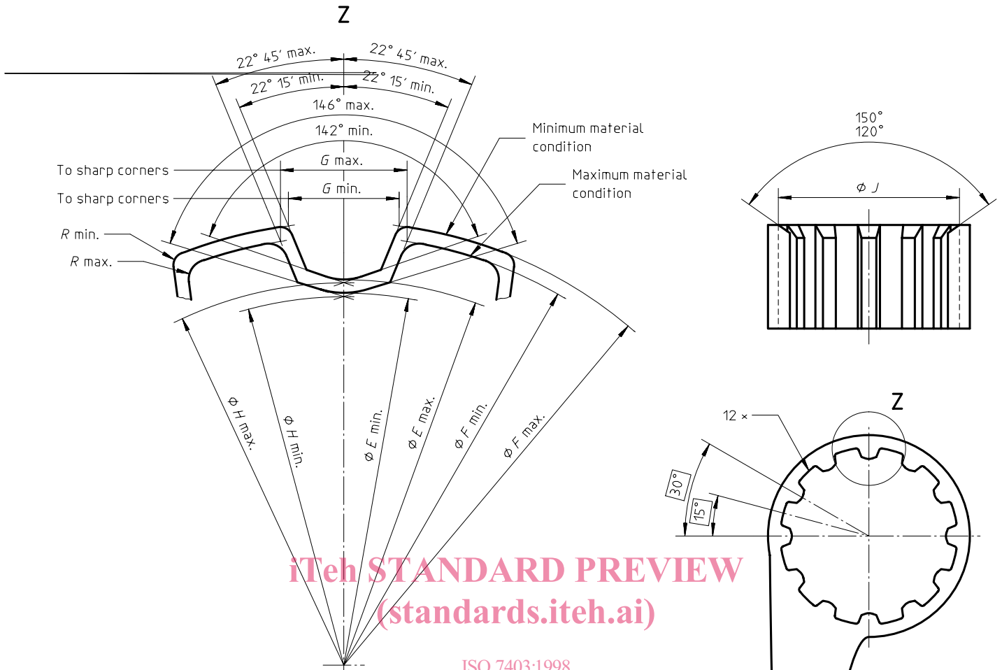
ISO 7403:1998 https://standards.itech.ai/catalog/standards/sist/33efd2cf-861c-4384-b850-7403 Figure 2 — Configuration 740 Internal spline drive
