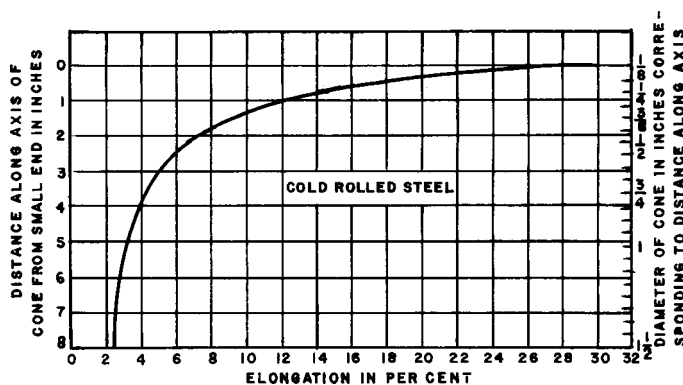
FIG. 2 Distance Along Cone and Corresponding Mandrel Size versus Percent Elongation for Specimens on Cold-Rolled Steel 0.8 mm (1/32 in.) in Thickness
