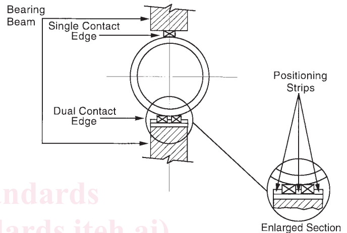
FIG. 2 Loading Apparatus
