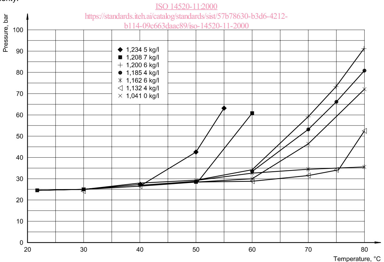
Figure 1 — Temperature/pressure graph for HFC 236fa pressurized with nitrogen to 25 bar at 20 °C
