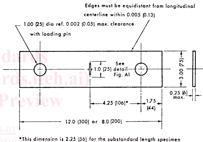
FIG. 3 Machined Sharp Edge-Notch Specimen, DE(T)
