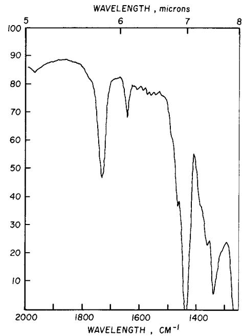
FIG. 1 Calibration Curve, 1 % Plasticizer in PVC Resin at 5.8 μm
