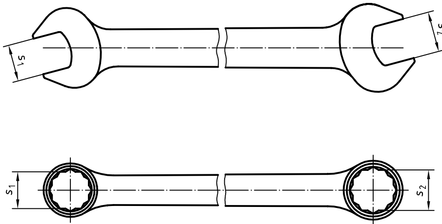
Figure 1 — Double-ended wrenches
