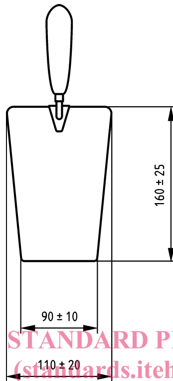
SIST EN 12350-4:2009 https://standards.iteh.ai/catalog/standards/sist/c72a6c98-acfd-4ab6-aa45-cc72cf0fad4a/sist-en-12350-4-2009 Figure 1 — Trowel
