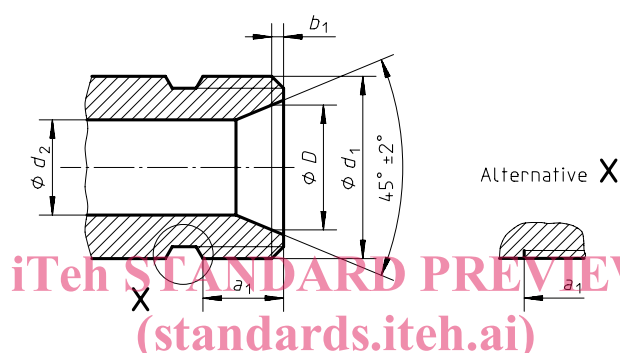
Figure 2 — Threaded union ISO 3253:1998
