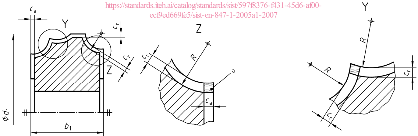
Figure 2 — Cutting diameter and cutting width
