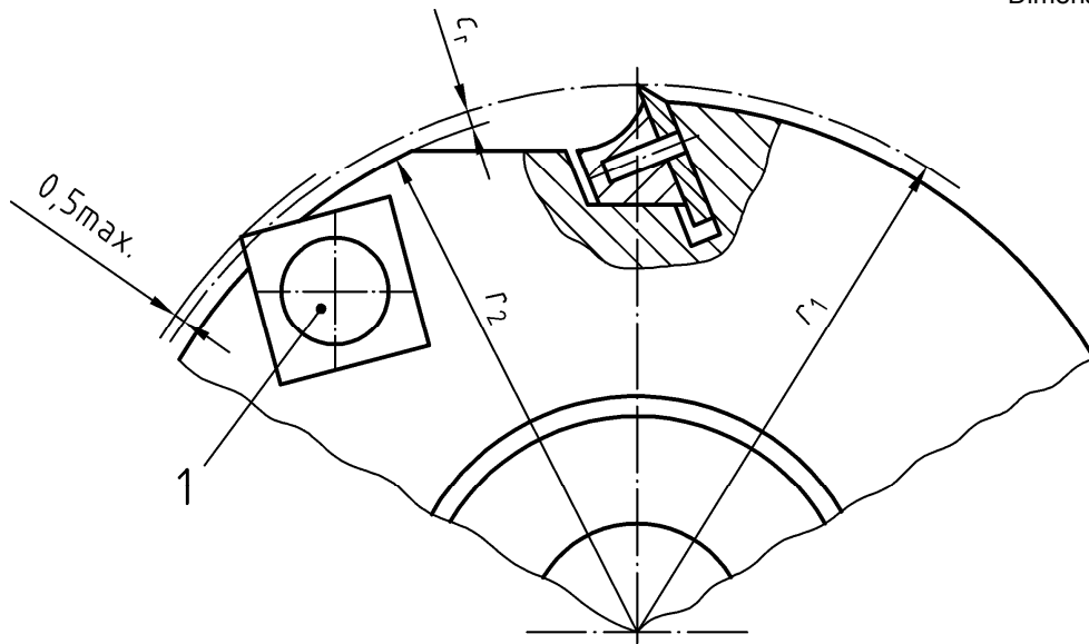
Figure 1 — Milling tool with a spur
