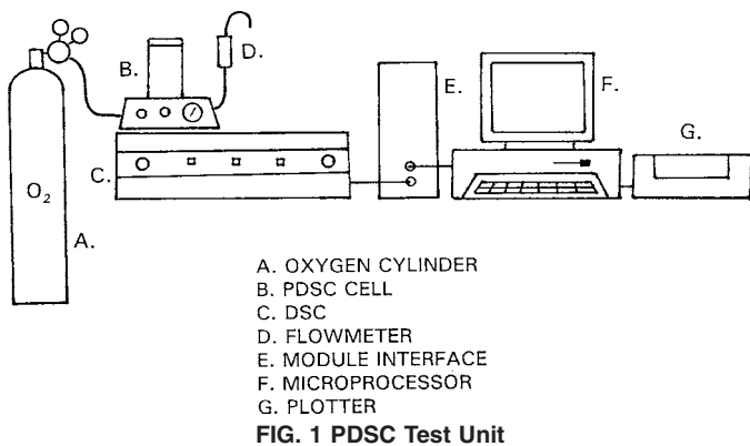
FIG. 1 PDSC Test Unit
