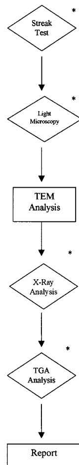
FIG. 1 Block Diagram of Suggested Analysis Scheme for Samples
