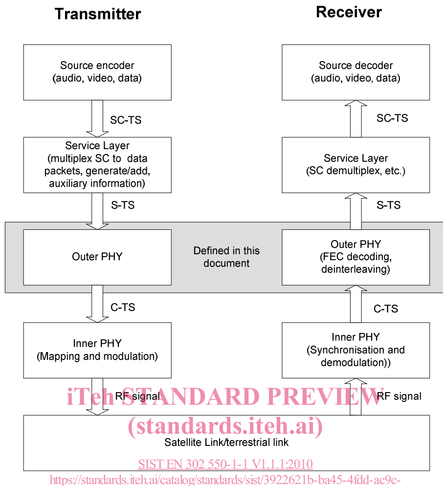
Figure 1: Position and interfaces of the OPL inside the transmission chain
