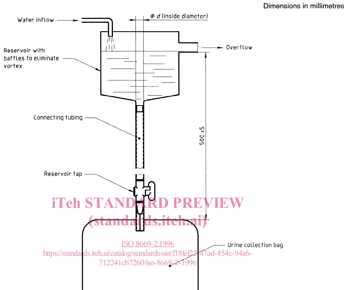
Figure 1 — Filling system for determination of test volume
