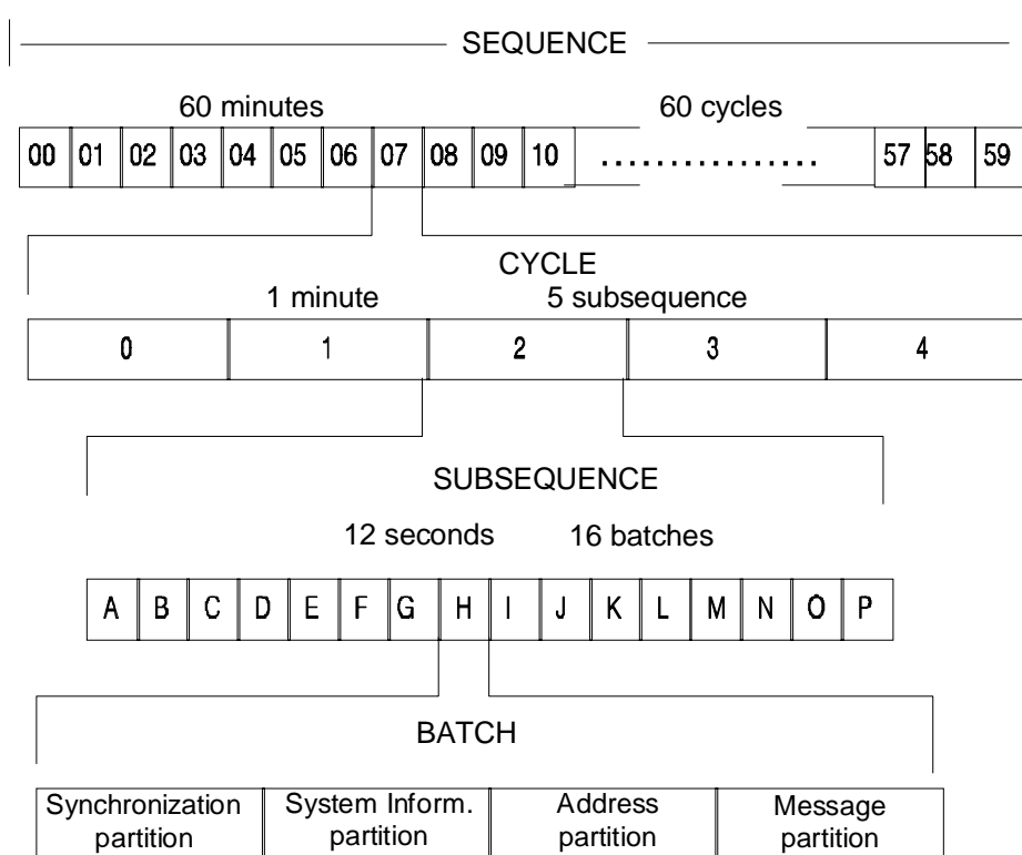
Figure 2: Structure of the radio protocol on channel one iTeh STANDARD PREVIEW (standards.iteh.ai)
