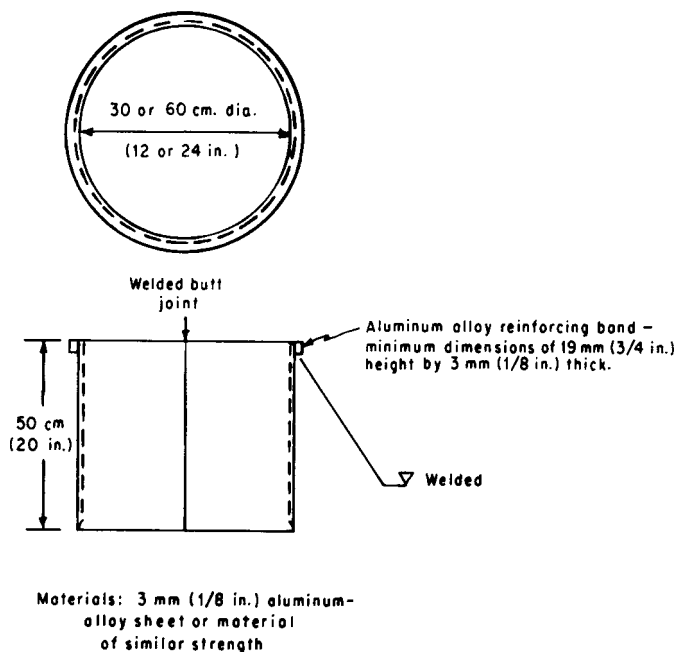
FIG. 1 Infiltrometer Construction
