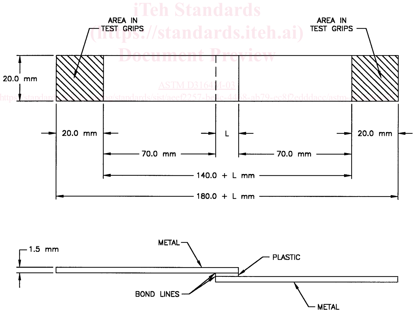
FIG. 1 Form A—Dimensions of Test Specimen
