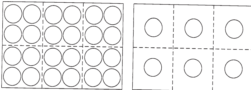
FIG. 5 Patty Positions for Heavy- and Light-Load Tests on a 36 by 24-in. (915 by 610 mm) Broiler Grate
